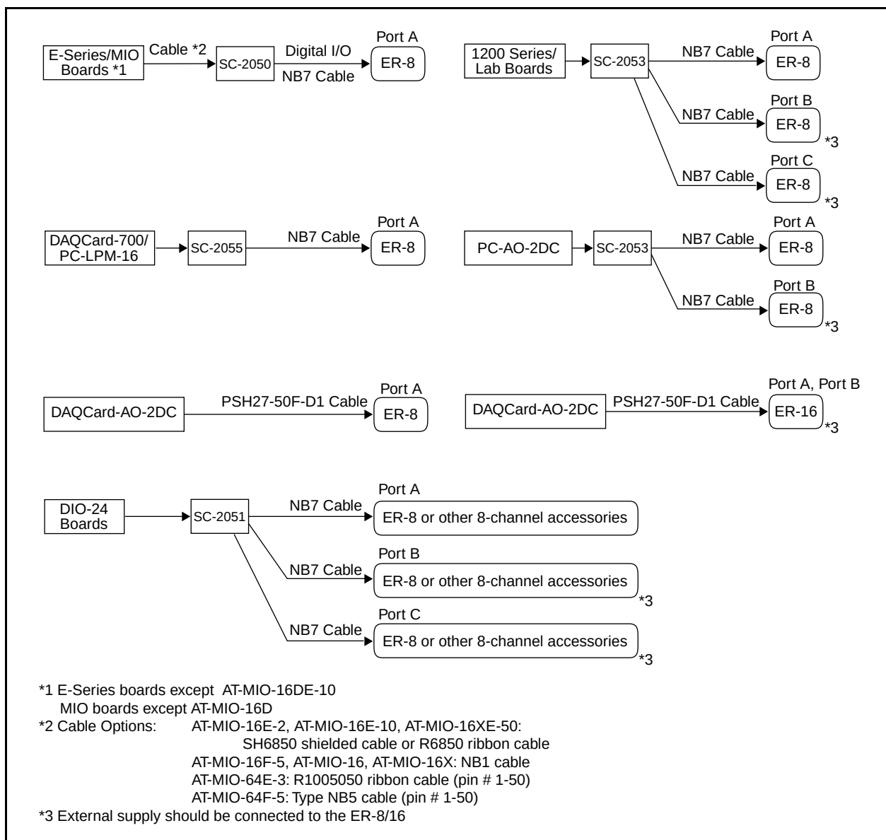
Figure 3-4. ER-8/16 Configurations with Multifunction DAQ Devices
