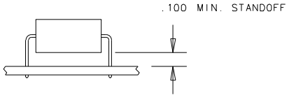
SXM350 DETAIL
