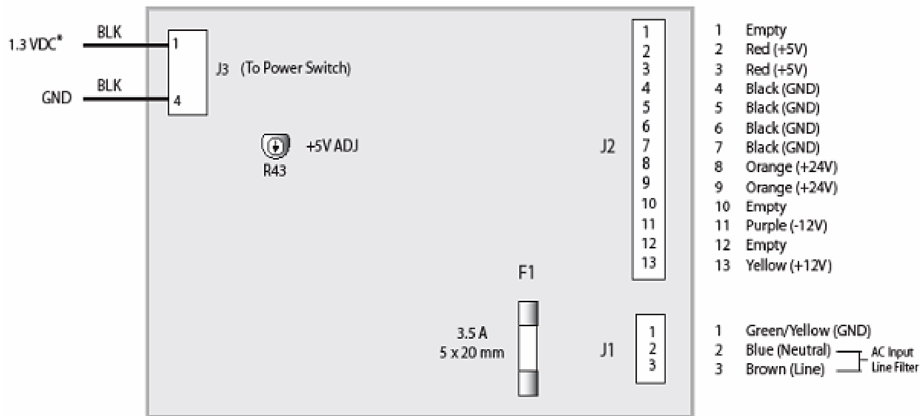
2489 UV/Vis Detector Low Voltage Power Supply Connections (Block Diagram)
