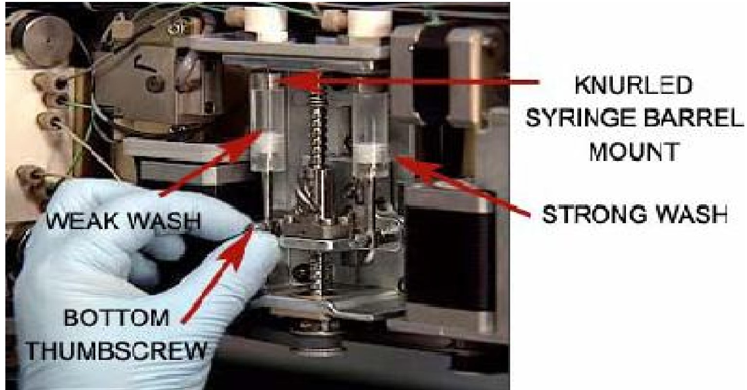
Location of Bottom Thumbscrew and Knurled Syringe Barrel
