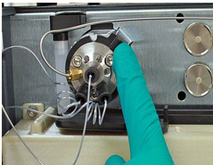
Outlet Switching Valve (low pressure fittings)
