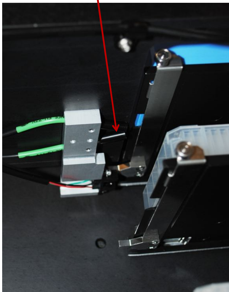
Micro-titer Plate Sensor
