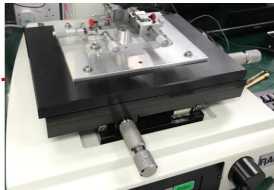
999043875 - PDA Alignment Fixture
