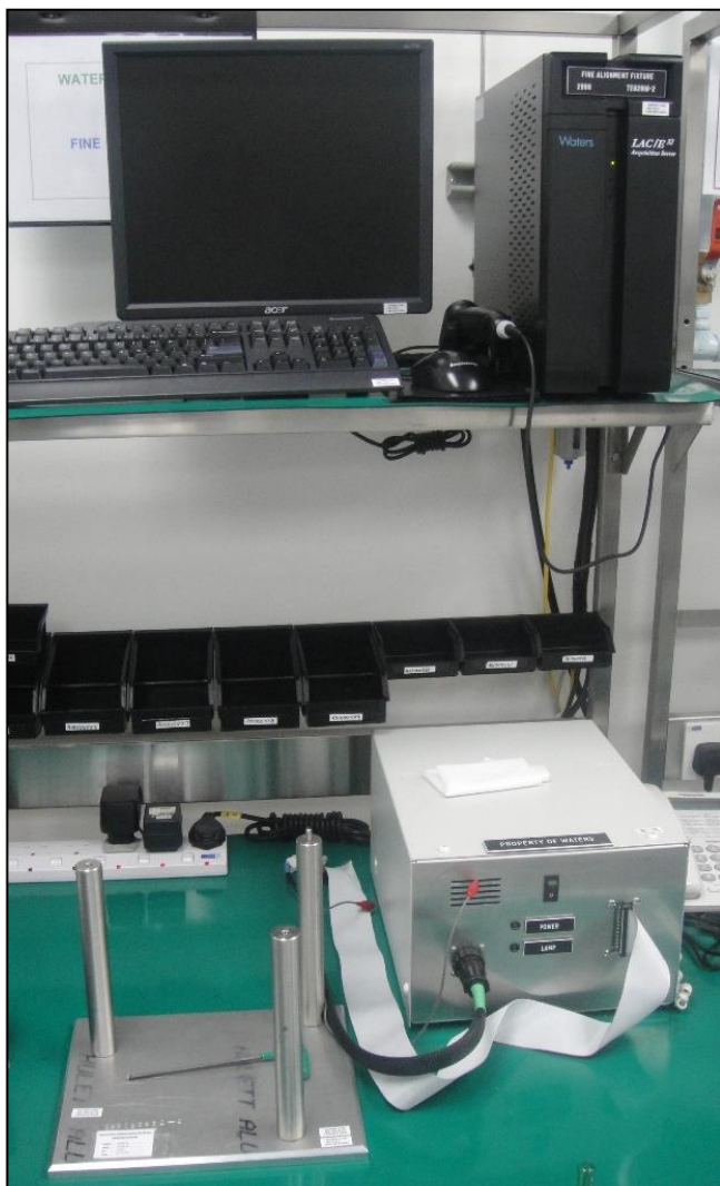
TE82918 Fine Alignment Fixture, Test System and PC Overview
