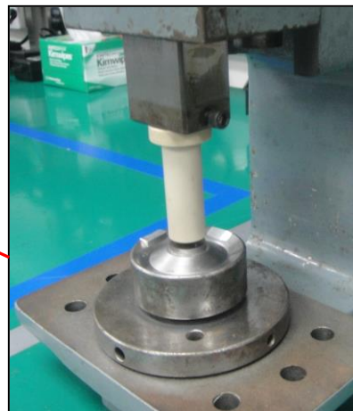
Peek Punch Assembly Fixture
