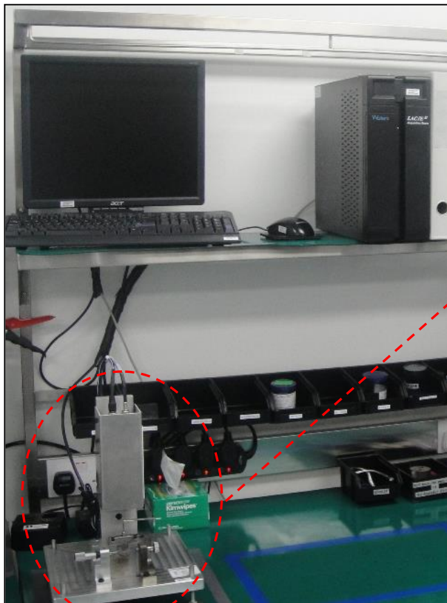
TE82868 Aperture Fixture and Test PC
