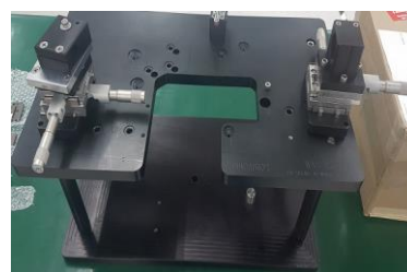
Rough Alignment Fixture
