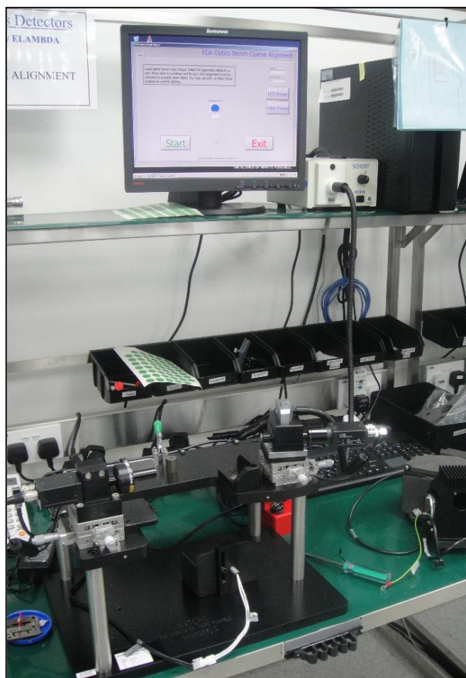
TE82880-2 Rough Alignment Fixture with Test PC
