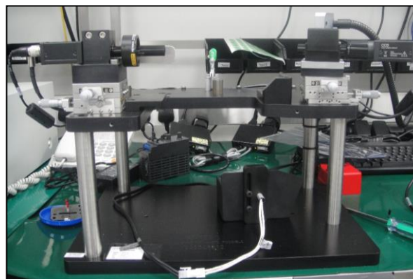
Rough Alignment Fixture
