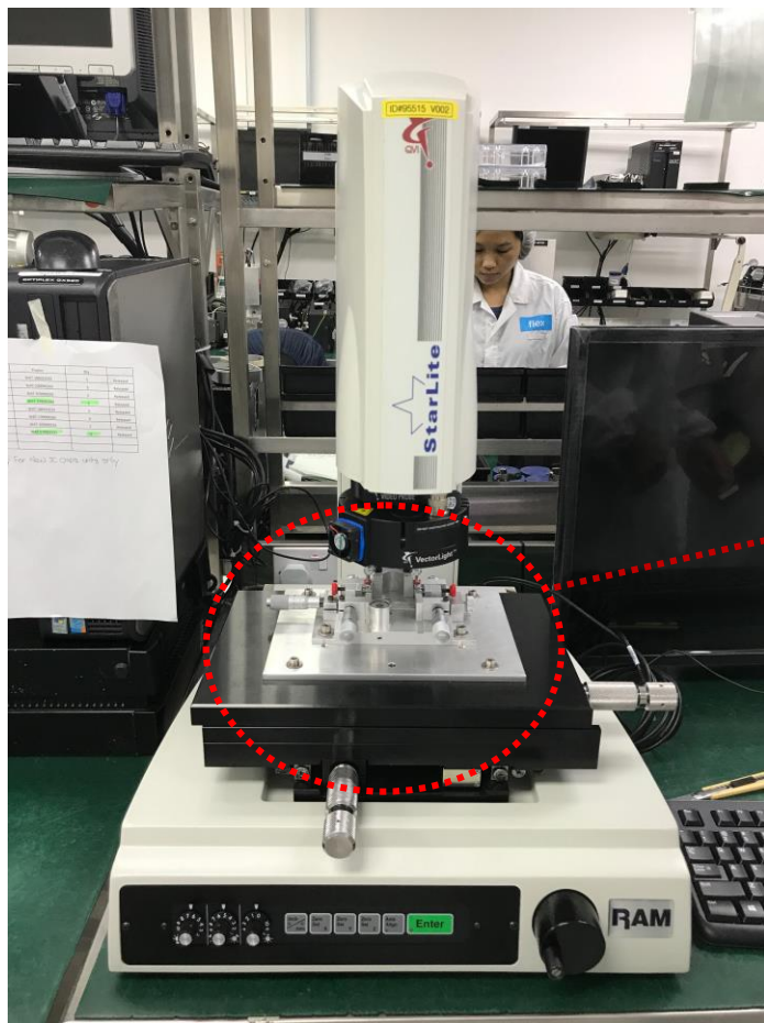
Starlite 150 - Optical Measurement System
