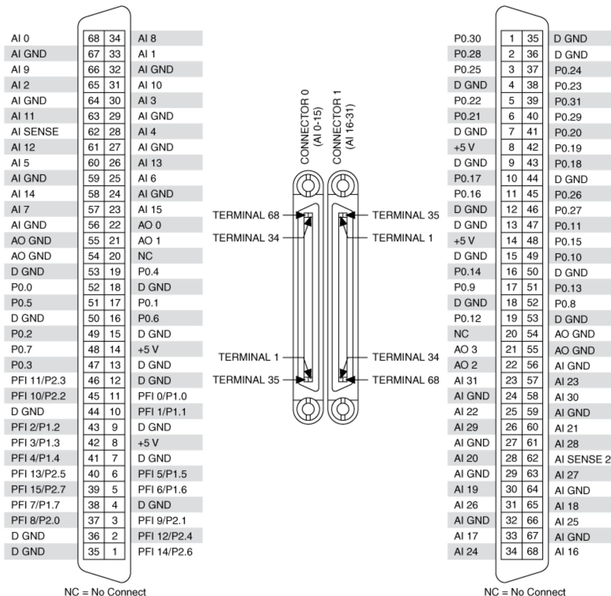
PCI/PXI-6229 Pinout
