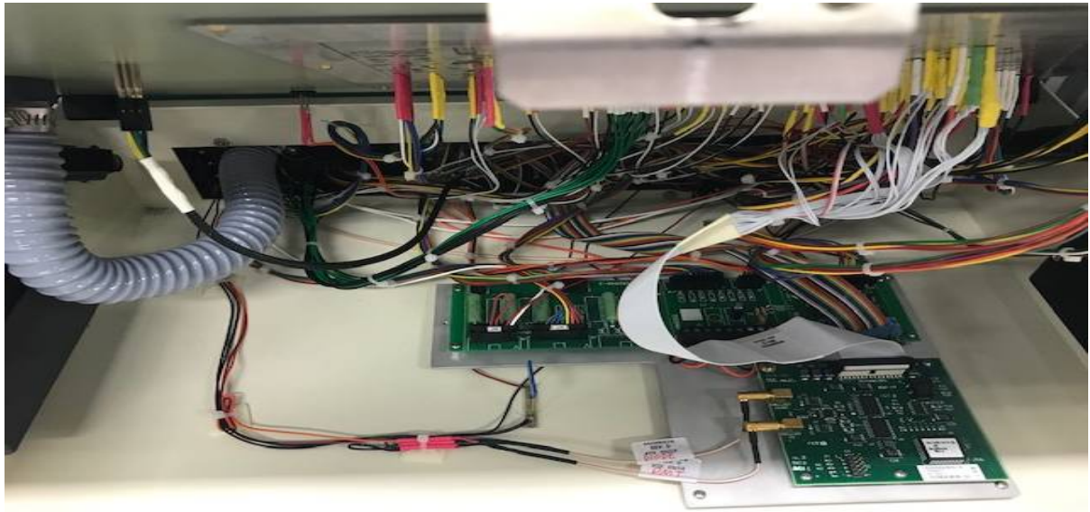
Inside FCT Test Fixture
