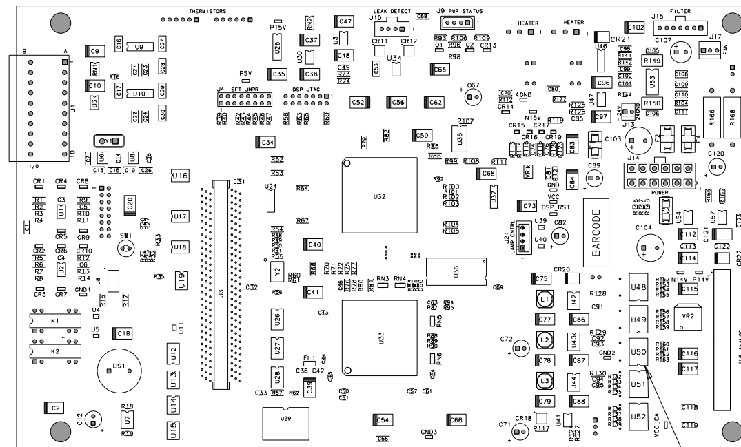
PRIMARY SIDE
