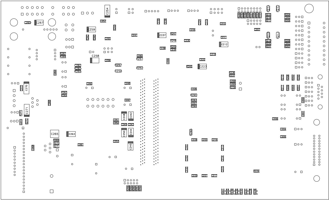
ASSEMBLY BOTTOM SIDE
