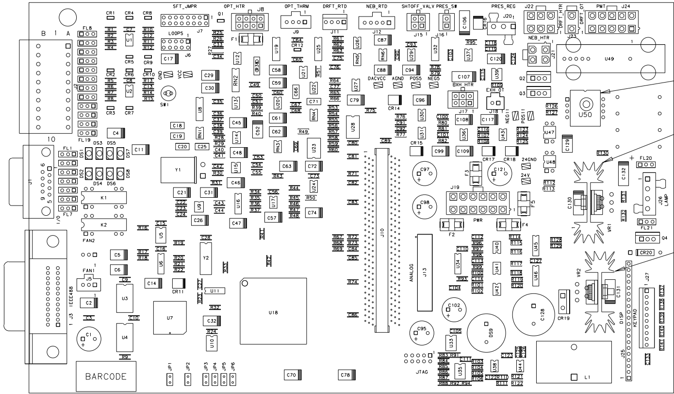
ASSEMBLY TOP SIDE
