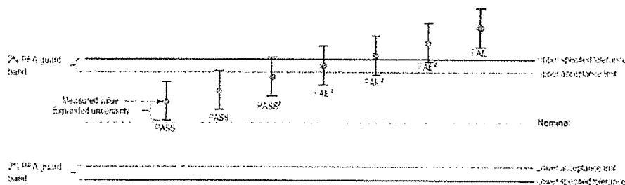
Acceptance limits for \leq 2\% probability of false accept (PFA) guard band
