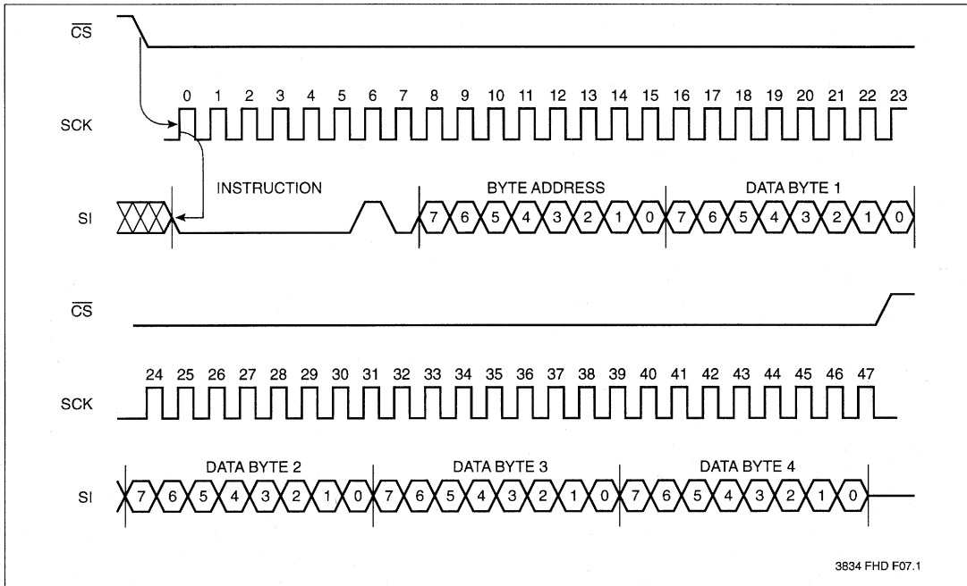
Figure 5. Page Write Operation Sequence
