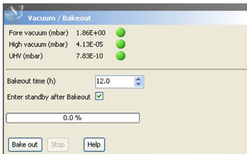
Figure 4-46. Vacuum / Bakeout window
