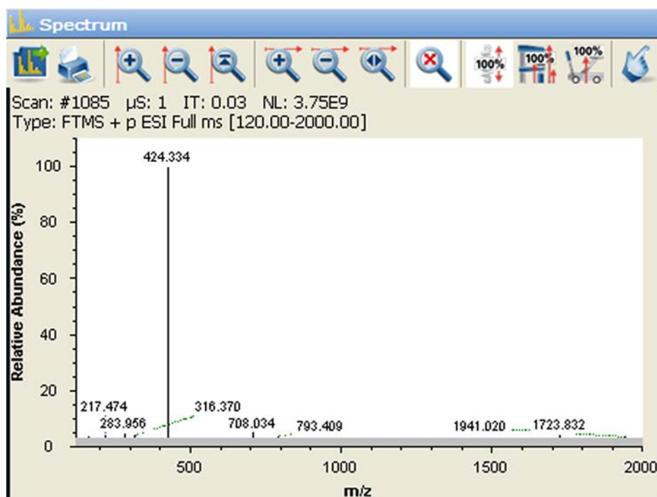
Figure 4-22. Spectrum window
