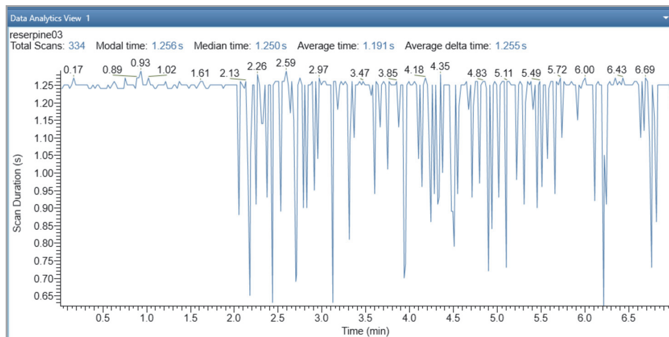
Figure 125. Scan Time
