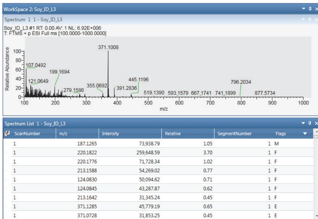
Figure 170. Spectrum List view (bottom) associated with the mass spectrum (top)
