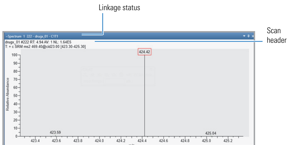
Figure 102. Spectrum view
