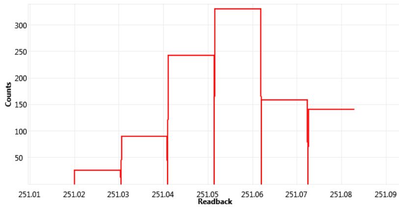
Q2_X Readback Histogram, Target: 251
