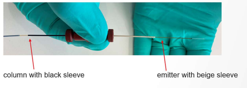
Figure 110: Complete Column and Emitter assembly
