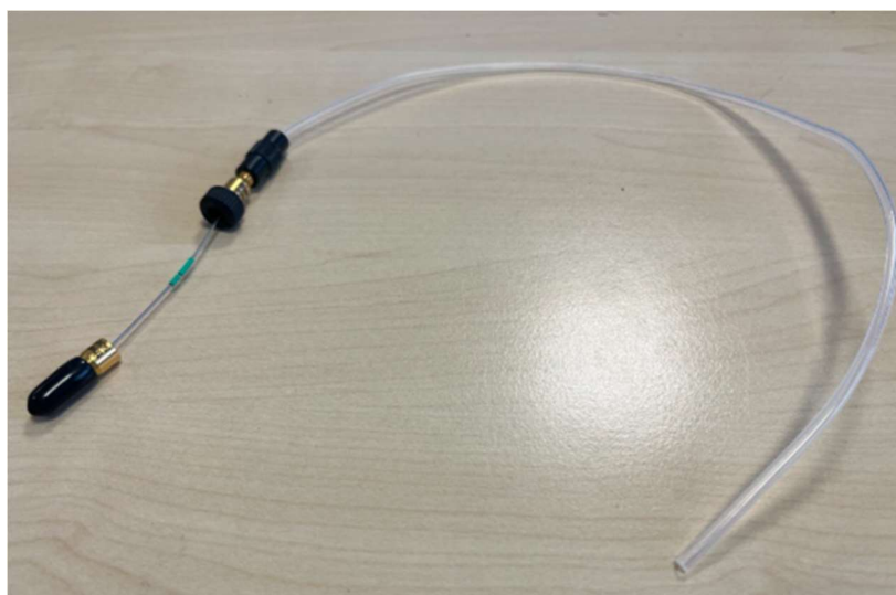
Figure 87: Waste line capillary which permits flow meter purging on the separation pump (P/N 6079.2425). The capillary is shipped with 2.5 meters of FEP (Fluorinated Ethylene Propylene) waste tubing which should be cut to the appropriate length prior to first use
