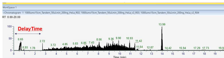
Figure 124: Elution profile prior to delay time adjustment
