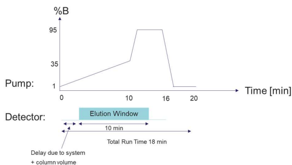
Figure 122: Schematic depicting gradient pattern for the test run
