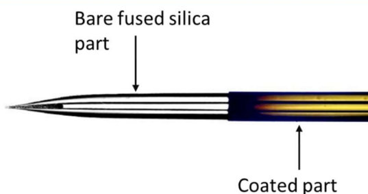
Figure 107: Parts of the Pulled ESI emitter (Figure taken from www.coannotech.com )
